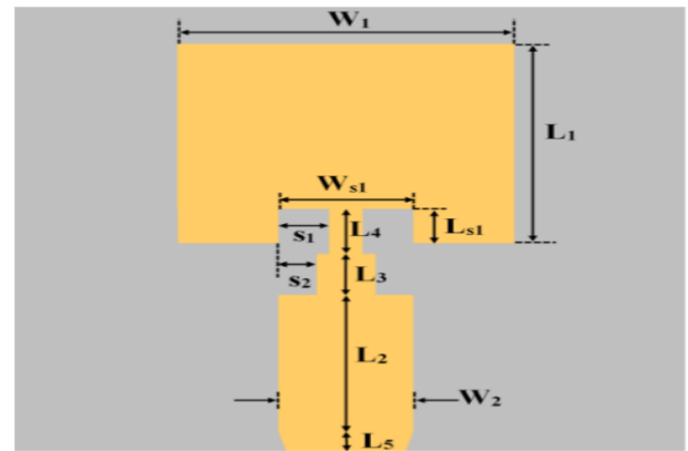
Fig. 1. Geometry of the patch antennas.
